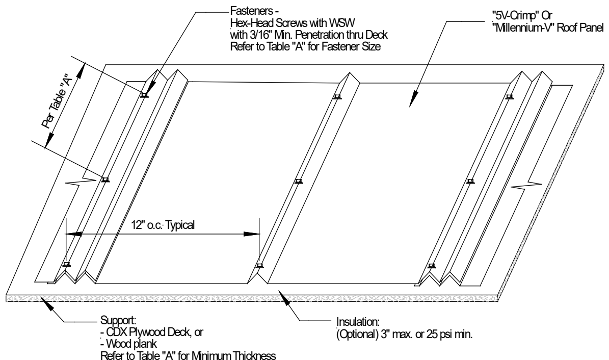
Drawing A-2 Typical Assembly Isometric View (Not To Scale) (Attachment METHOD 1, METHOD 3 & METHOD 4 Per Table "A")
