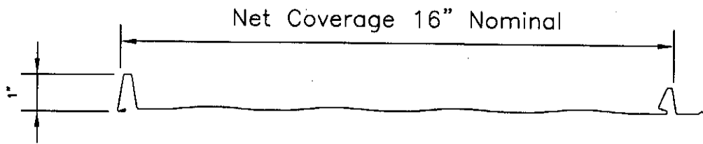
M-SEAM STRIATED PANEL PROFILE
