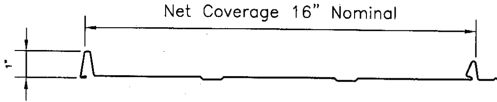
M-SEAM PENCIL-RIB PANEL PROFILE
