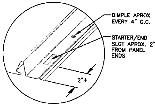
Nailstrip Detail
